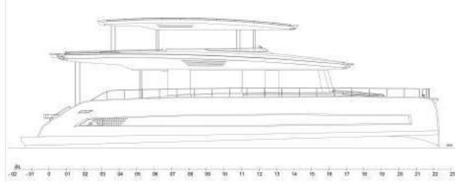
STB SIDE VIEW
