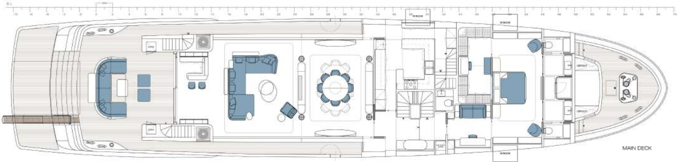
UPPER DECK
