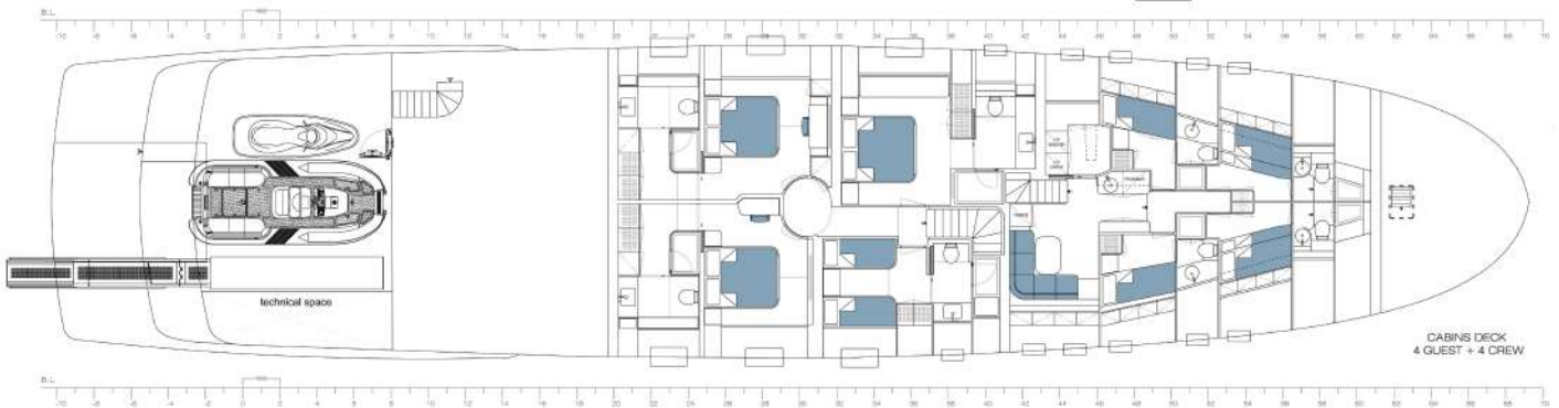
MAIN DECK
