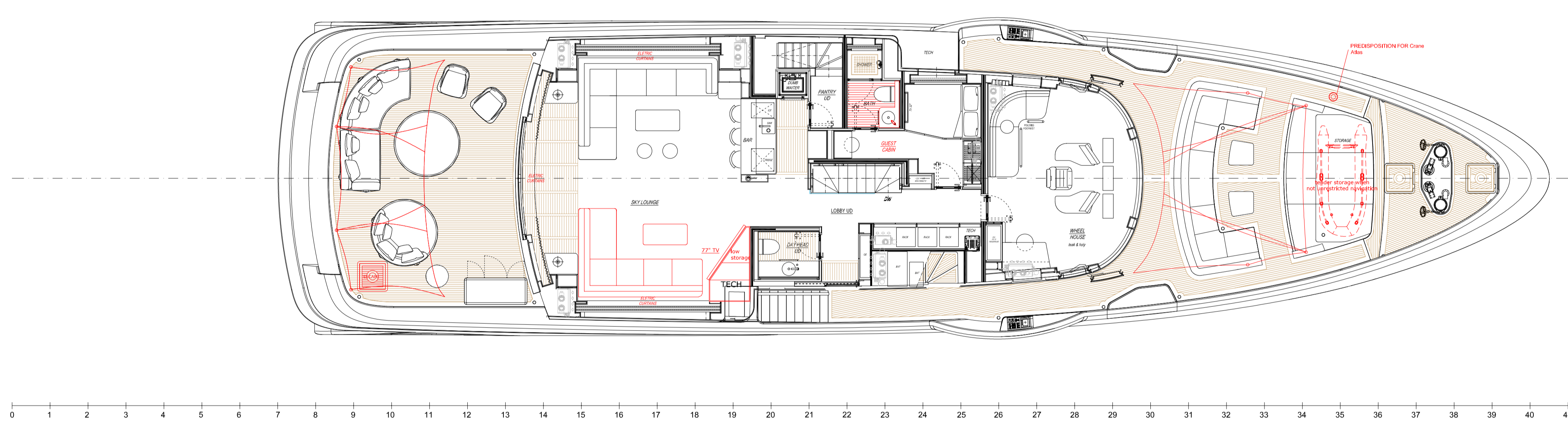
UPPER DECK
