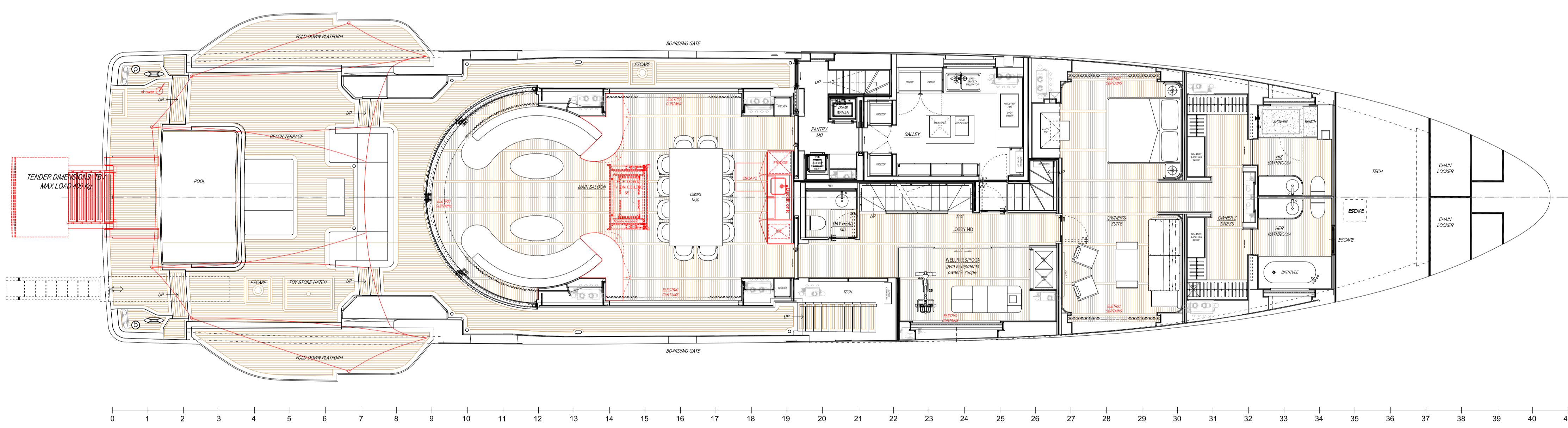
MAIN DECK
