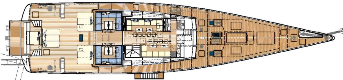
Main deck
