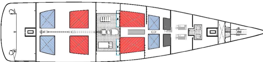
Bilge deck
