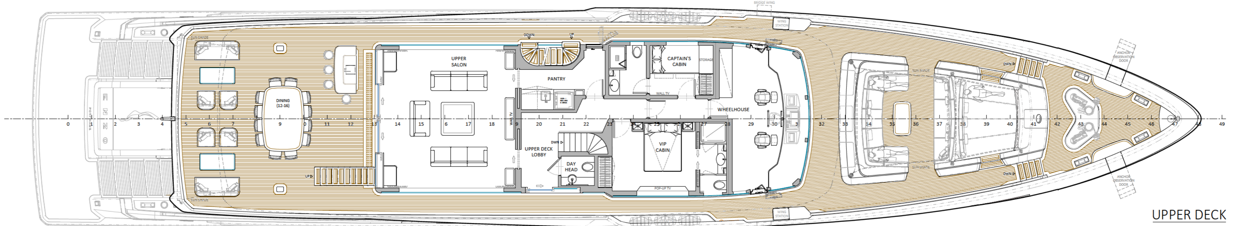
SUN DECK
