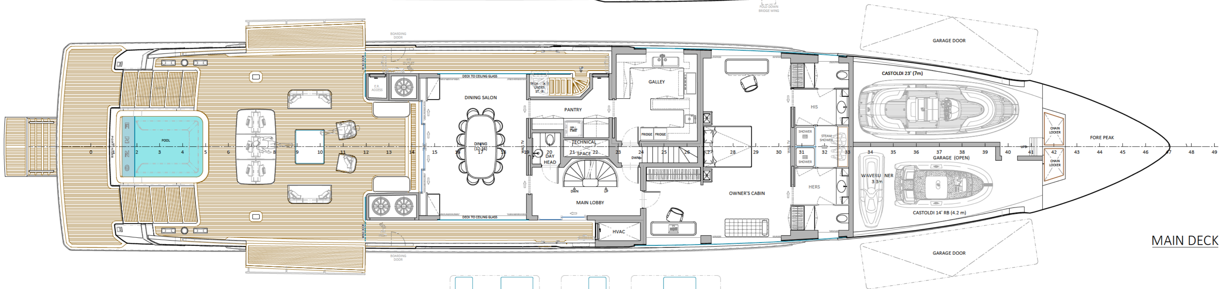
UPPER DECK
