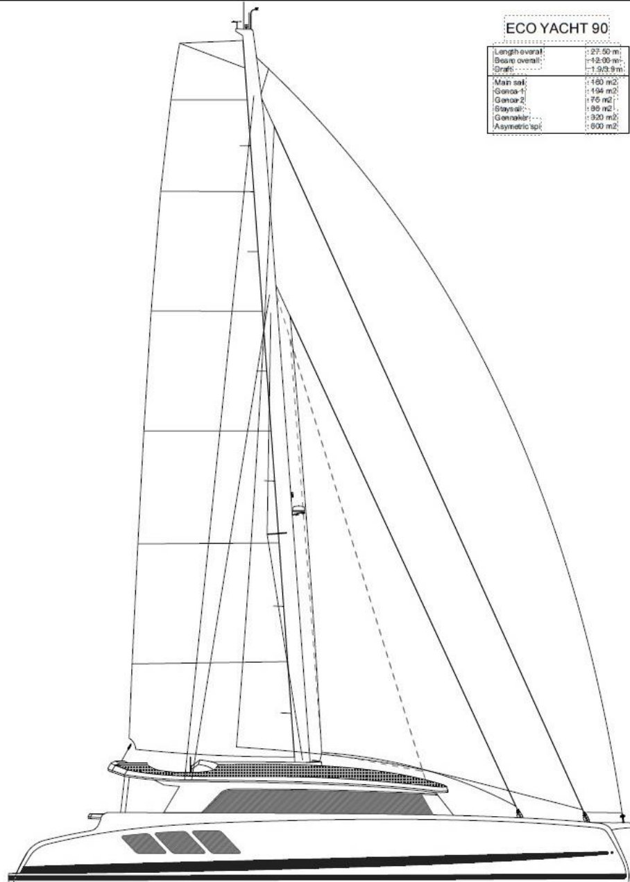
ECO YACHT 90-02 General profil View.
