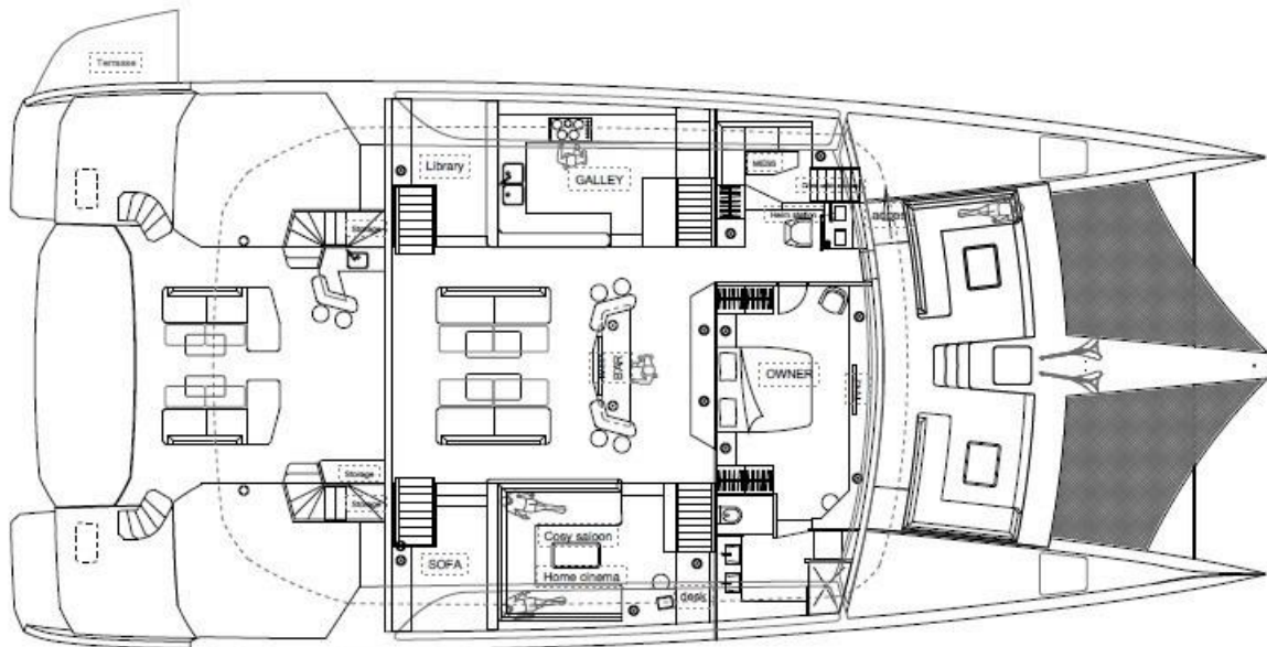
Plan view - Main deck v.2d:
